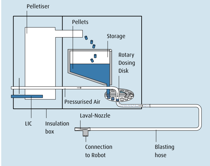
CRYOCLEAN® complete schematic.
